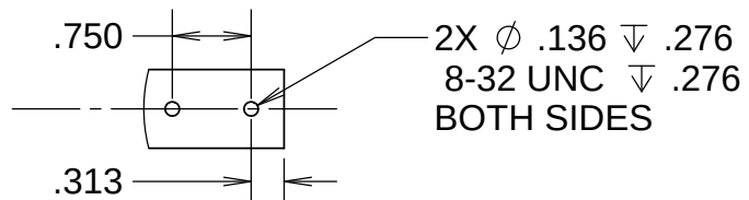
DETAIL J
