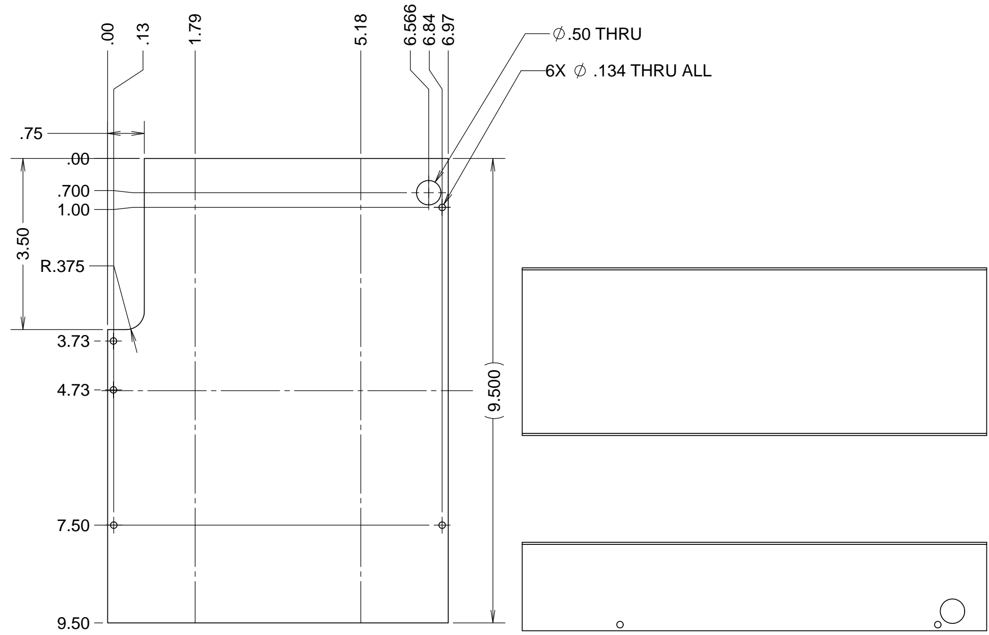
FLAT PATTERN
